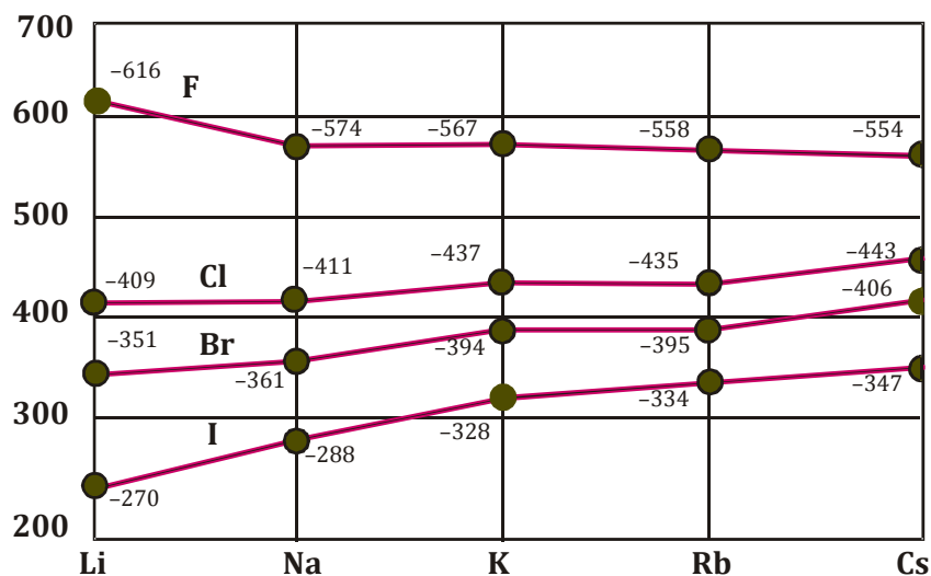
The standard enthalpies of formation of the halides of Group 1 elements at 298 K
